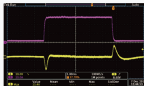
Paralleled units
