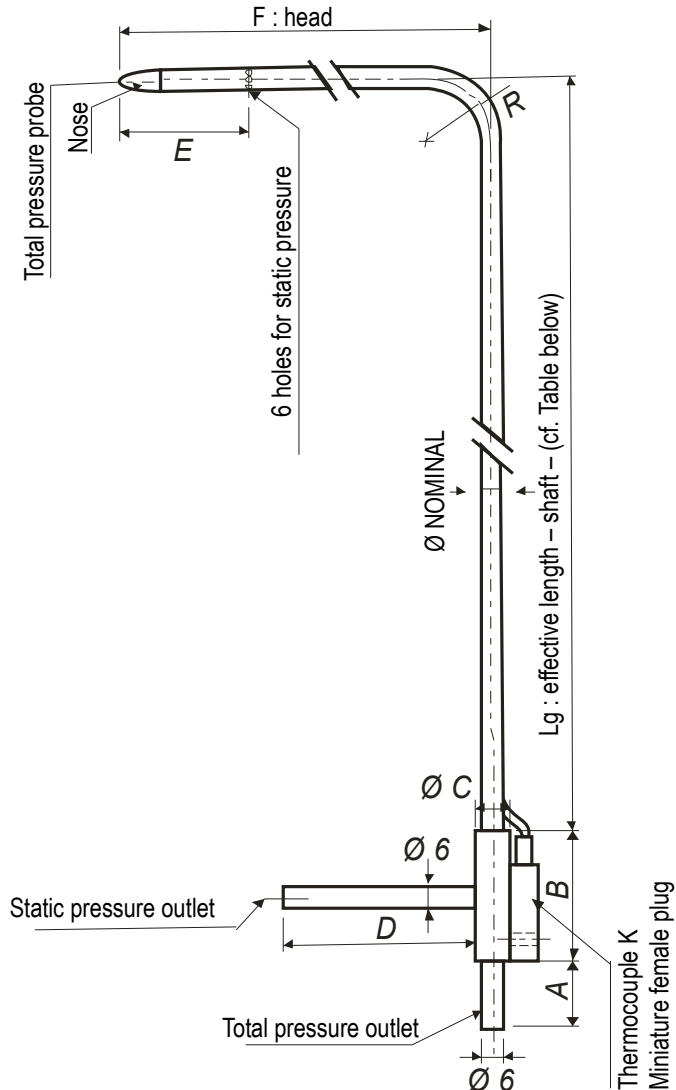
Pitot tube Type L with TC K
