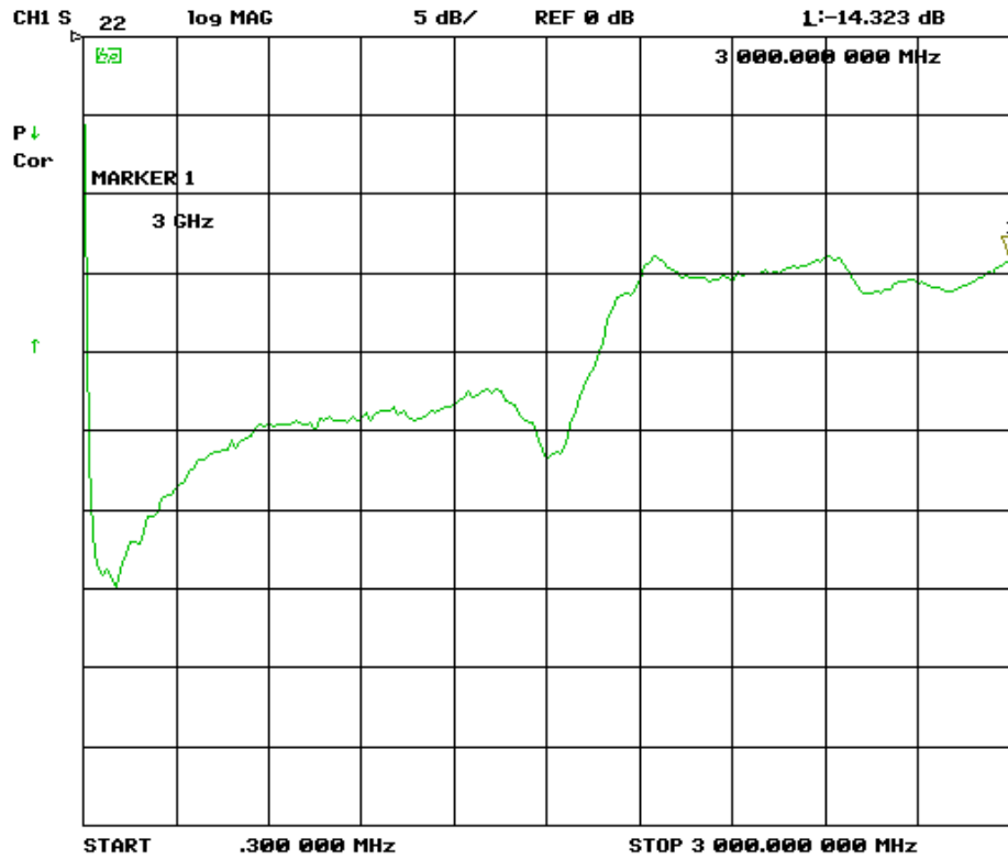
Picture 18 – TBWA1/40dB, output return loss, IS22I, 300 kHz – 3 GHz, lin.
