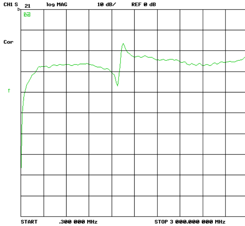
Picture 3 – H20, coupling loss, 300 kHz – 3 GHz, lin.
