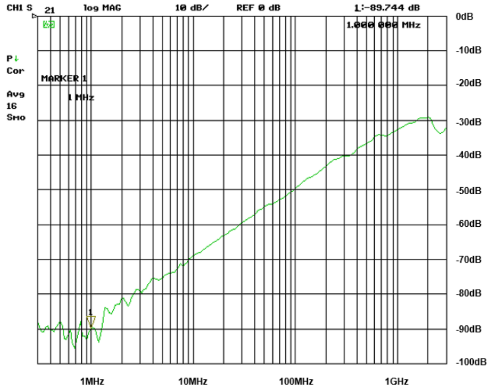
Picture 10 – E5, coupling loss, 300 kHz – 3 GHz, log.
