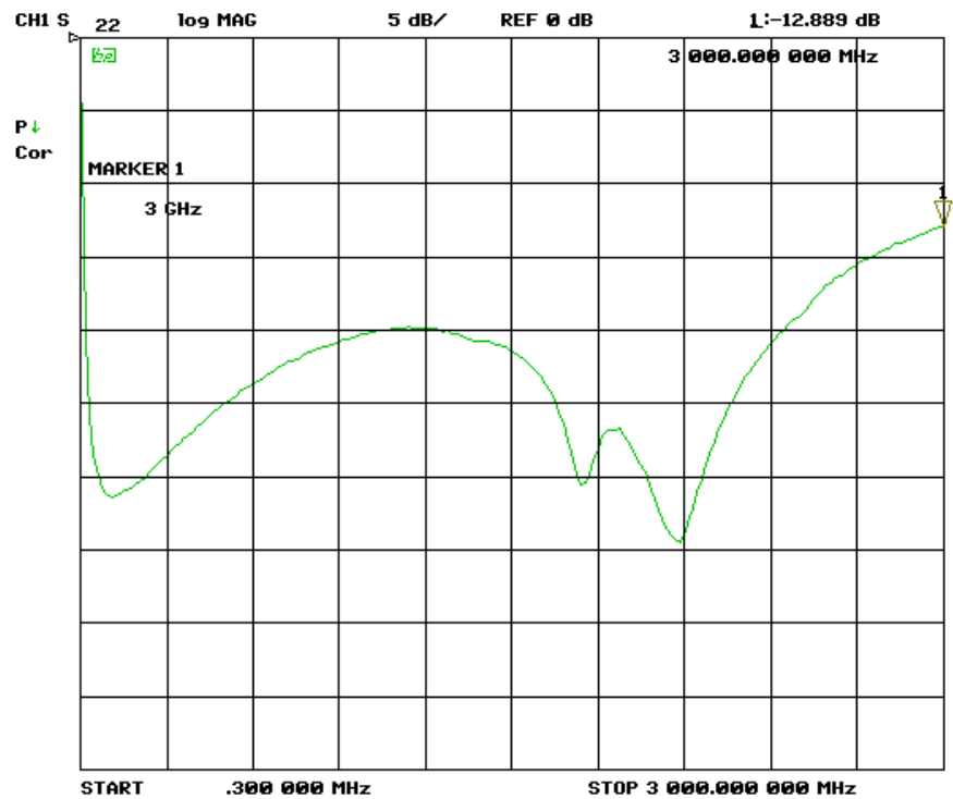
Picture 14 – TBWA1/20dB, output return loss, IS22, 300 kHz – 3 GHz, lin.
