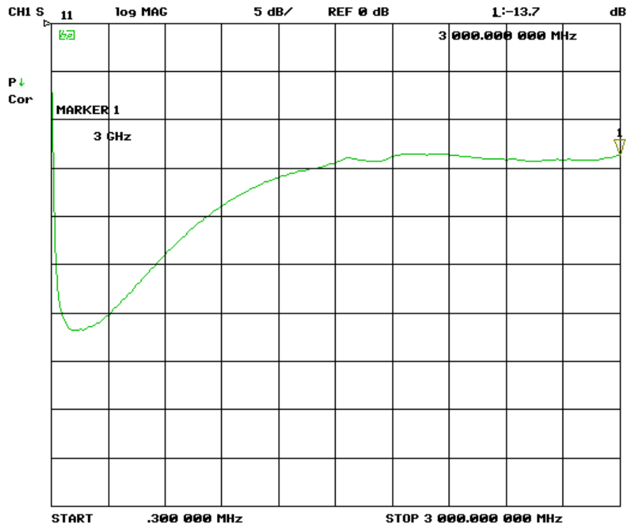
Picture 13 – TBWA1/20dB, input return loss, IS11, 300 kHz – 3 GHz, lin.
