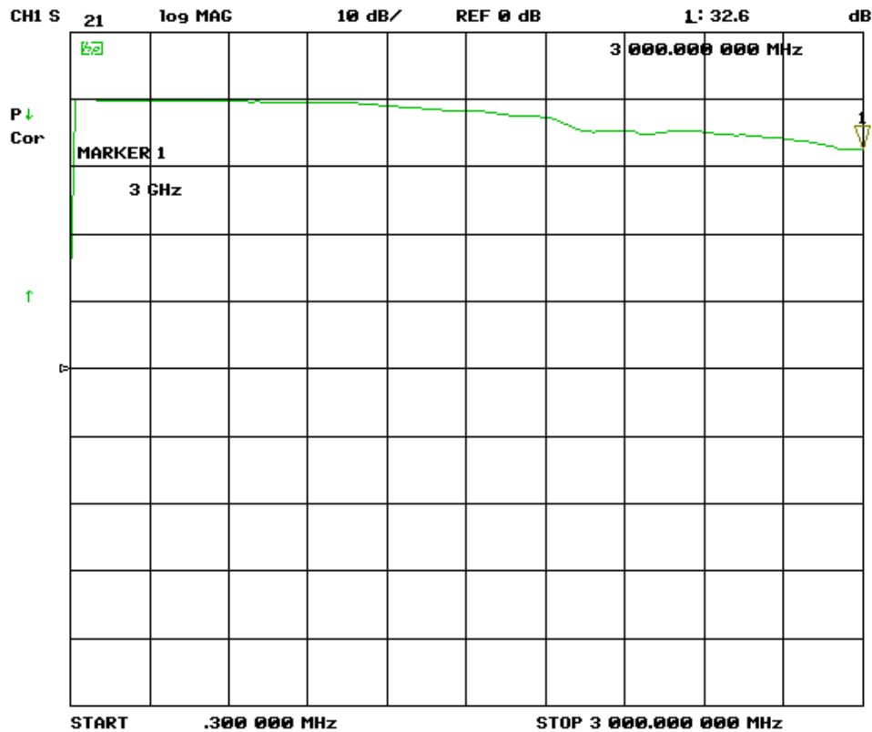
Picture 15 – TBWA1/40dB, gain, 300 kHz – 3 GHz, lin.
