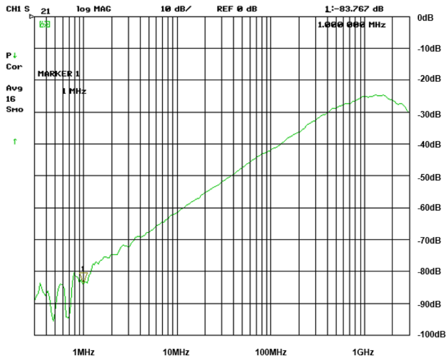
Picture 6 – H10, coupling loss, 300 kHz – 3 GHz, log.
