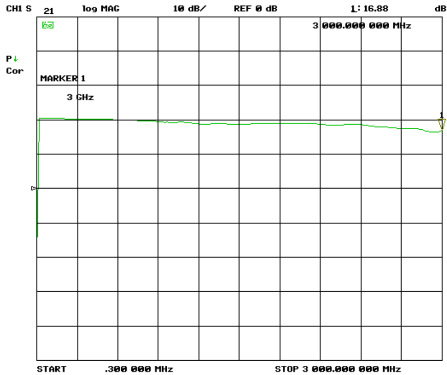
Picture 11 – TBWA1/20dB, gain, 300 kHz – 3 GHz, lin.
