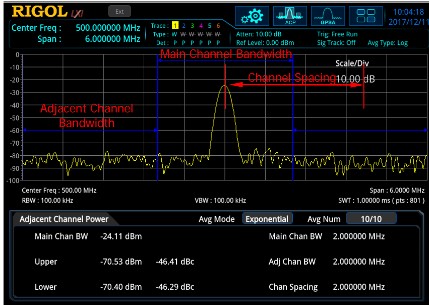
Figure 2-6 Adjacent Channel Power Measurement Interface
